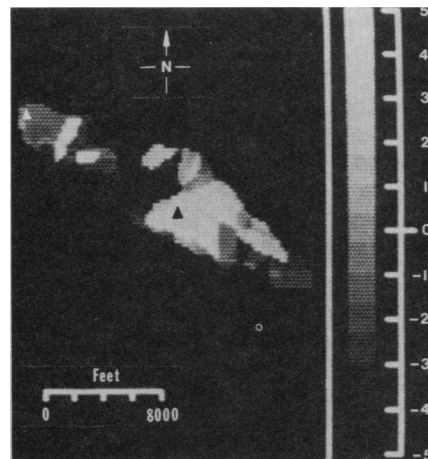
Fig. 4. The February 1980 PROSPECTOR evaluation for intense hood-type porphyry molybdenum mineralization based on prospecting and mapping which terminated in 1978. The favorability scale (-5 to +5) is brightness-coded as shown at the right. If the hood model holds, the map suggests either two separate deposits, structural modification of a single hood, or some other aberration. Because of the absence of data, the favorable zone terminates at the southeast end; the deposit may extend off the map area.
